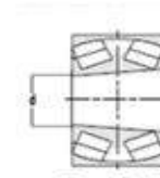
Tapered Bore (K) (1:12)
