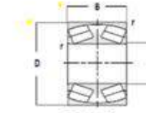
Cylindrical Bore
